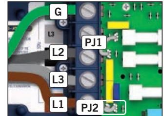
3-phase Delta (no neutral)
