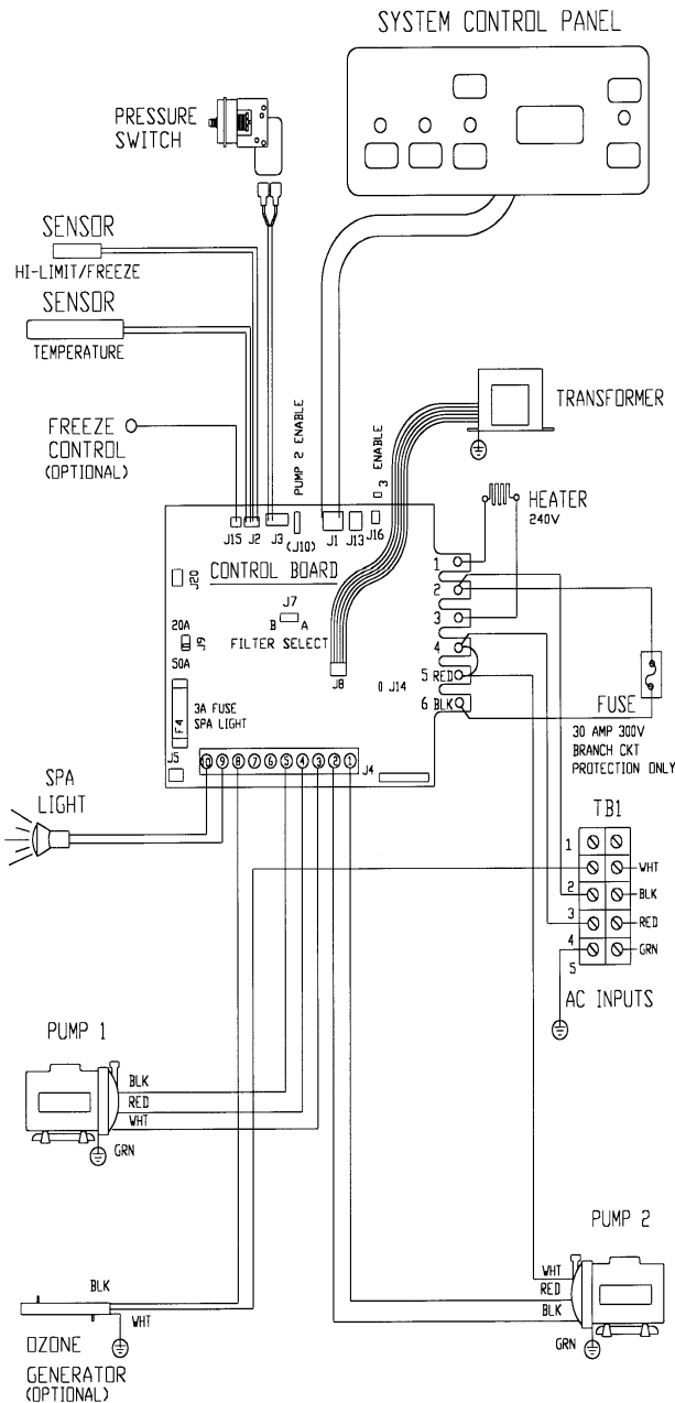
(Figure D) Deluxe 240V Wiring Diagram
